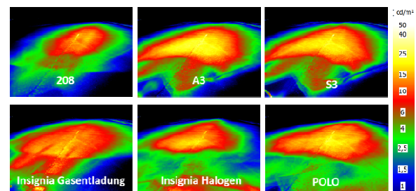
Figure 6: Luminance in the area in front of the test vehicles
